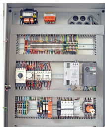
▶ Electrical Cabinet
